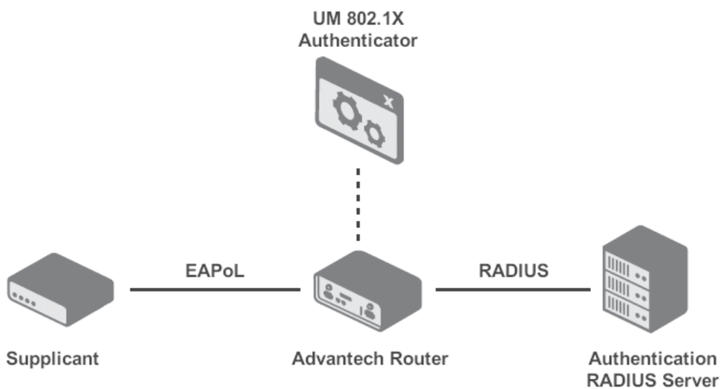
Figure 1: Functional Diagram
